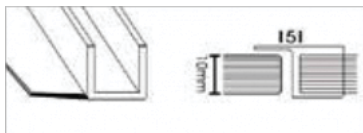
Glass To Glass 90° ( F profile)
